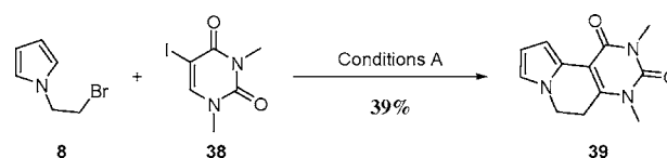
Scheme 3. Iodo-uracil 38 as the Iodo-Partner
