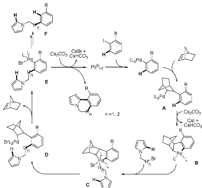
Scheme 2. Proposed Mechanism for the Synthesis of Annulated Pyroles
